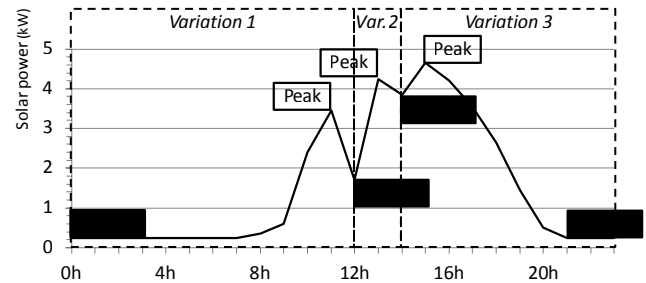
Figure 1: Three variations of solar power generation during a partly cloudy day in summer (produced with a 5 kW installation of photovoltaic panels, on the buildings' roof of our laboratory, on August 26, 2012).
